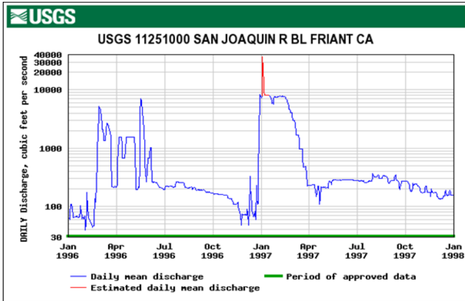
Figure 8. Hydrograph for water year 1997, San Joaquin River below Friant Dam, the largest flood event on record post dam construction.
