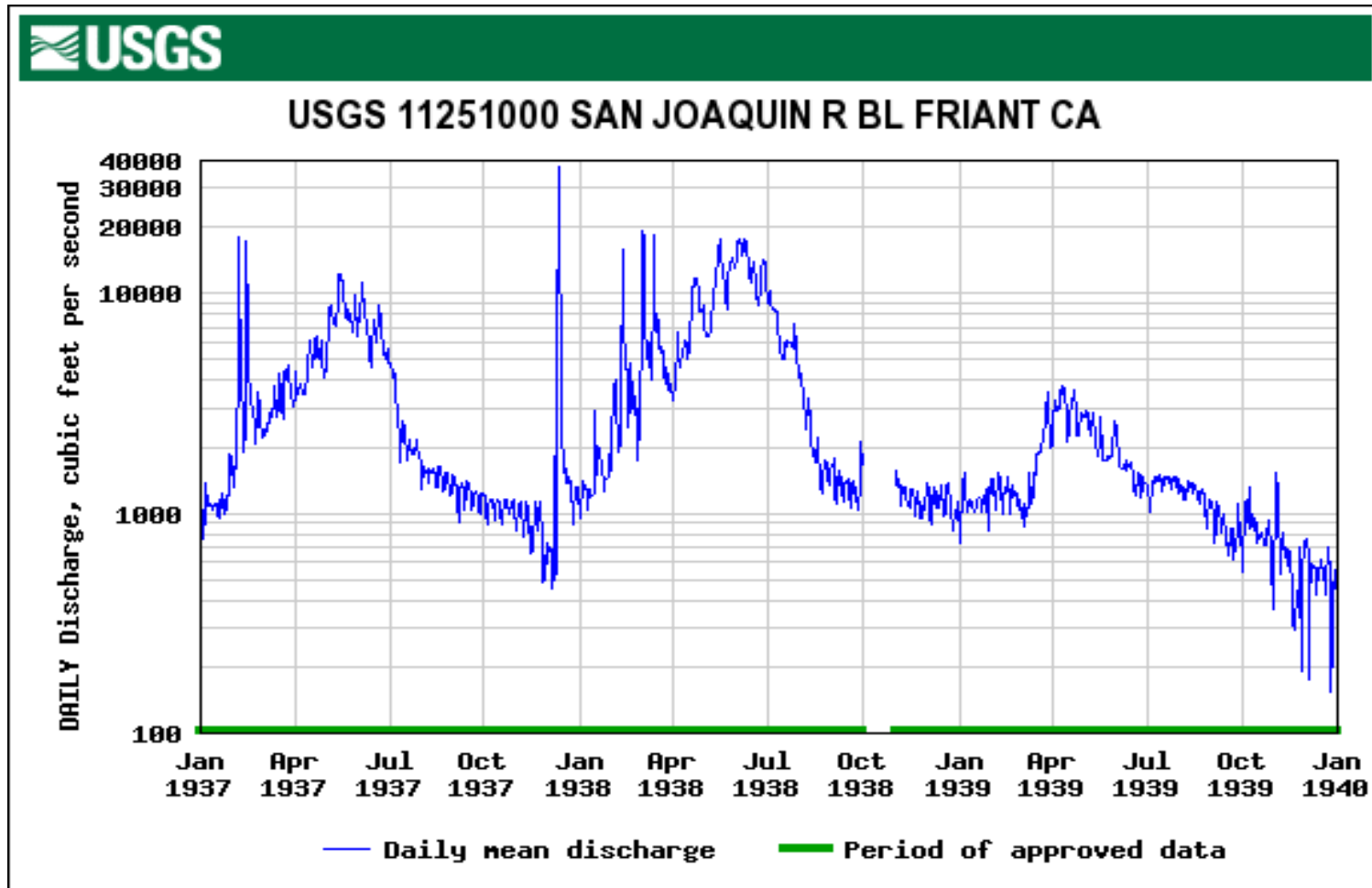
Figure 7. Hydrograph for water year 1937, showing the largest winter flood event prior to the construction of Friant Dam.
