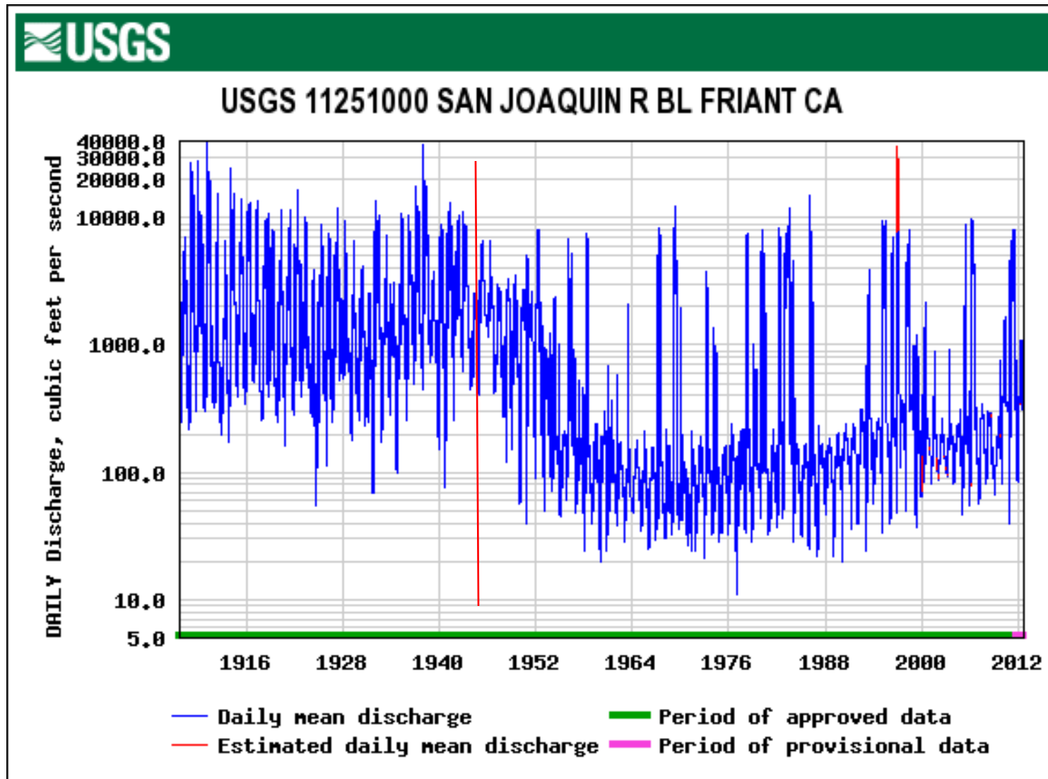
Figure 5. San Joaquin River stream flow below Friant Dam for the period of record 1907-2012. Vertical red line indicates 1944, the year Millerton Lake began to fill.
