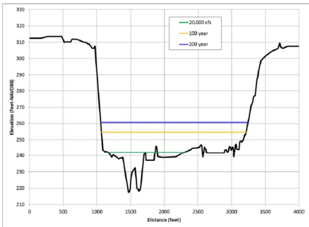
Figure 1: Comparison of water surface elevations from Board designated floodway flow (20,000 cubic feet per second), the 100-year flood (71,000 cubic feet per second) and 200-year flood (110,000 cubic feet per second) at the project location (Reference: see Attachment B, Exhibit D)
