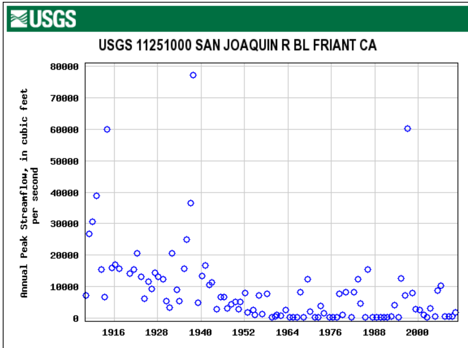
Figure 6. San Joaquin River annual peak stream flows below Friant Dam for period of record at gage #11251000.
