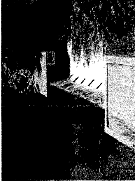
Photo D-56. Flashboards in place at Bonomo Flashboard Dam
