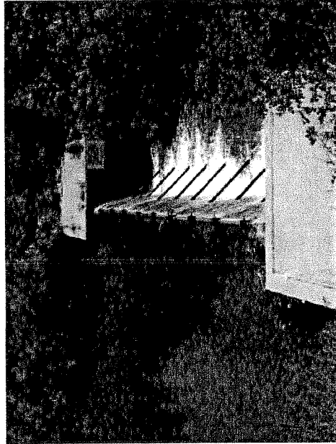
Photo D-86. Flashboards in place at Piazza Flashboard Dam Interstate 5 Bridges
