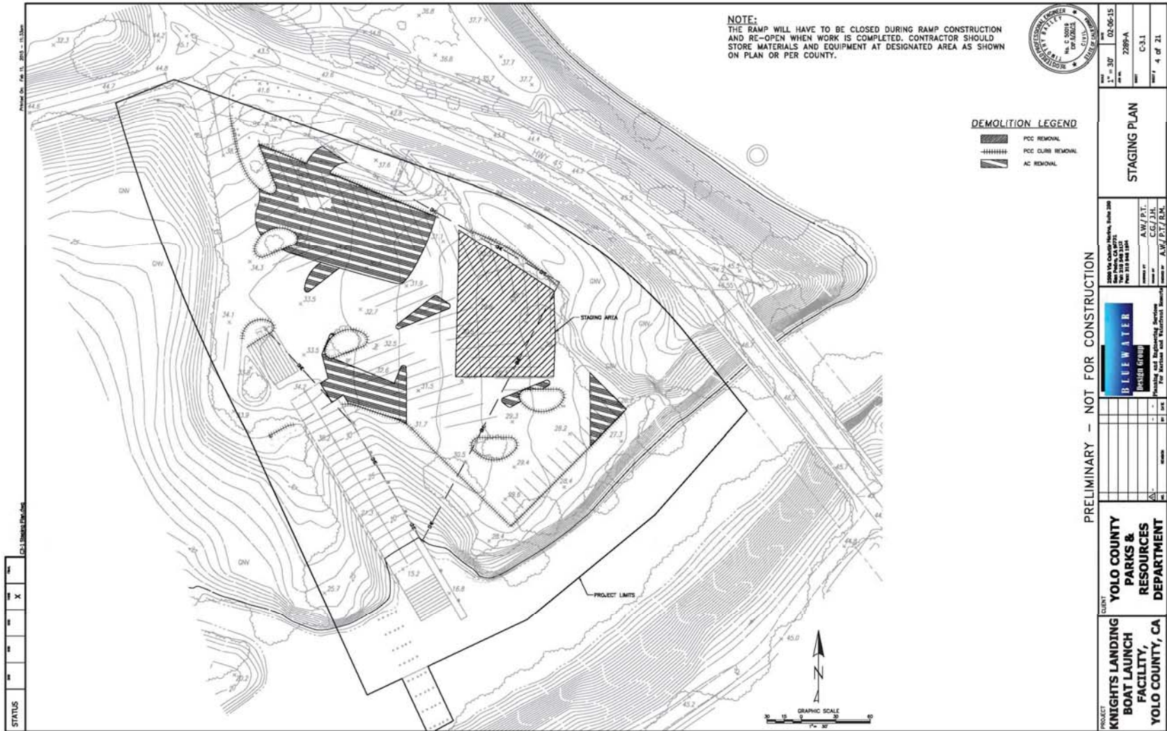
Figure 4 Staging Plan
