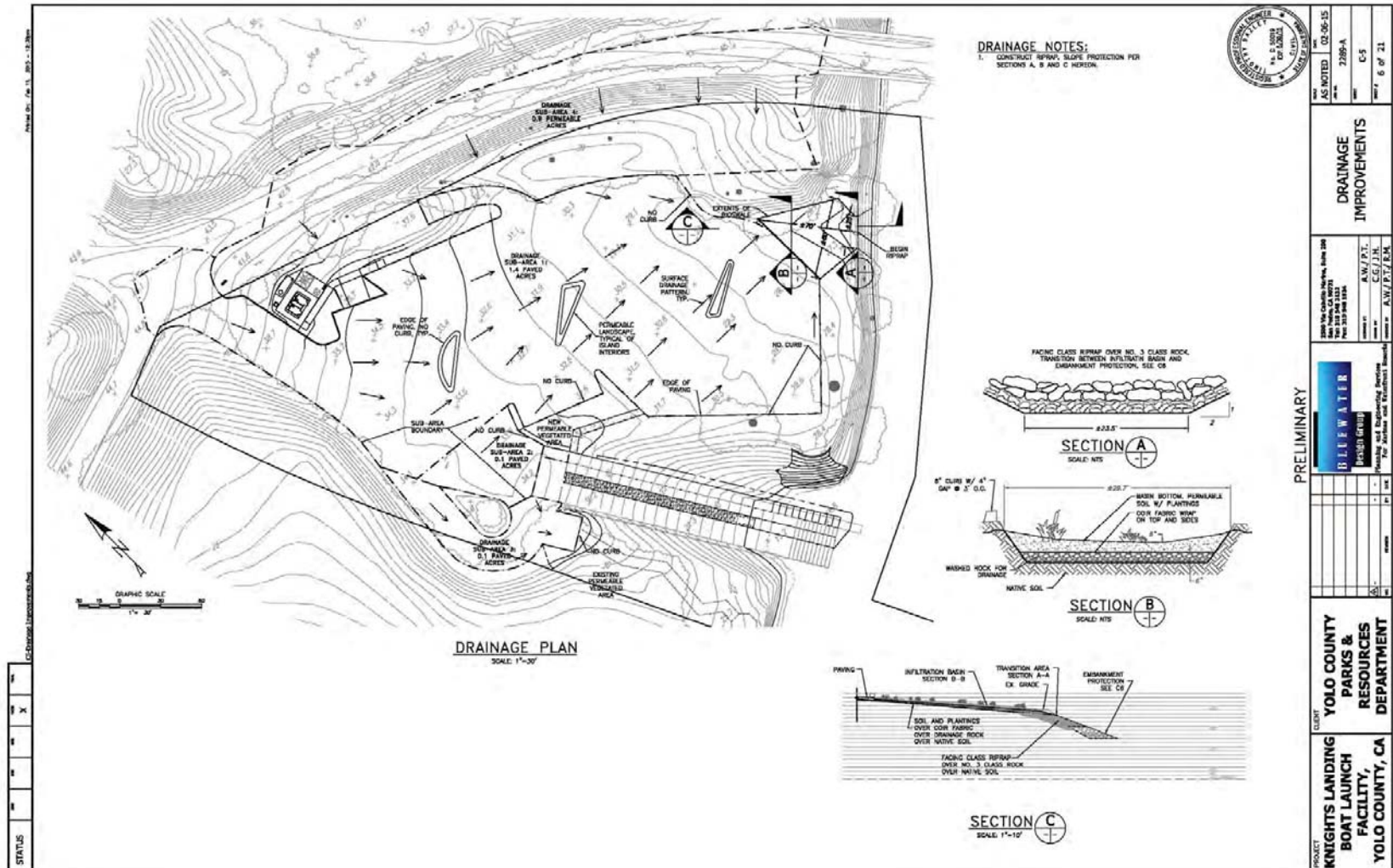
Figure 5 Drainage Improvements
