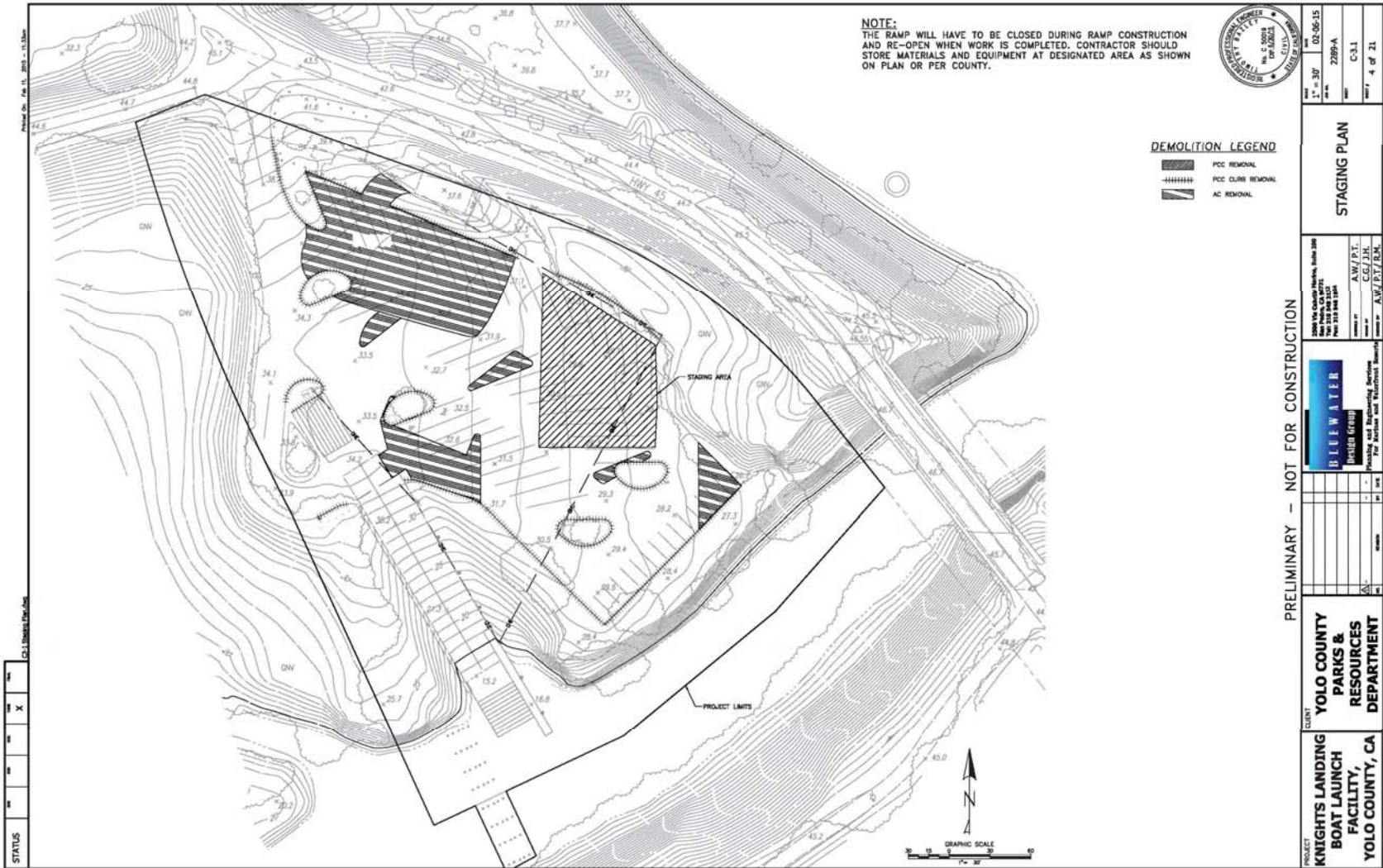
Figure 2 Staging Plan
